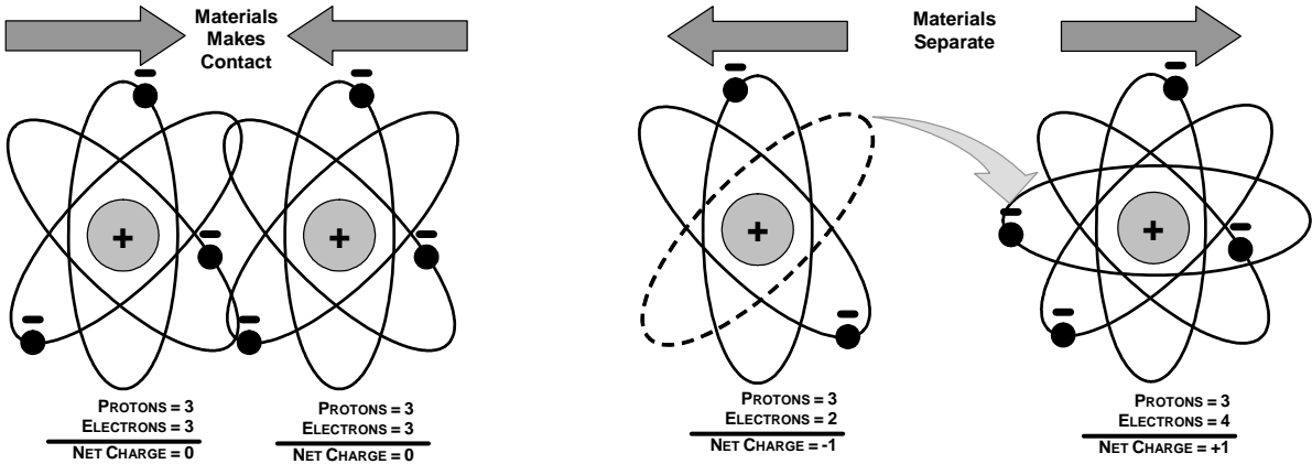
Figure 1-1: Triboelectric Charging
