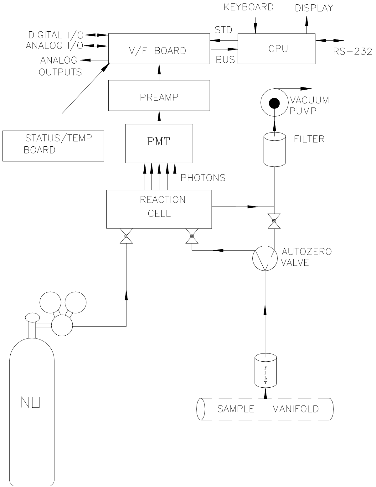
Figure 3-1: Block Diagram
